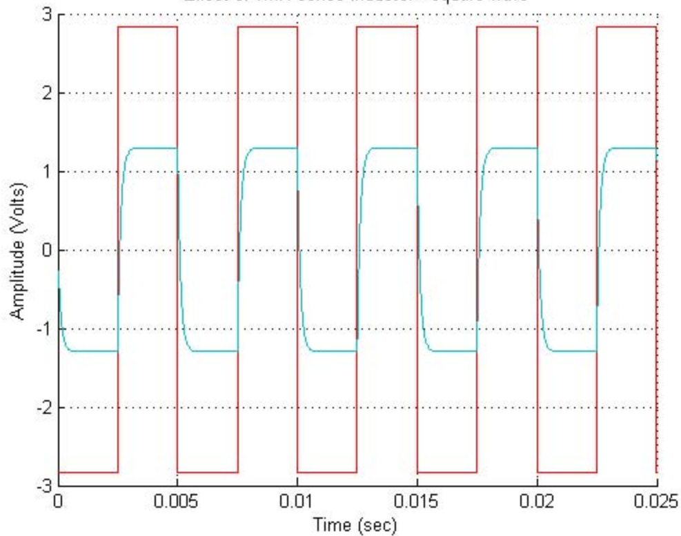
Effect of 1mH series inductor - square wave
