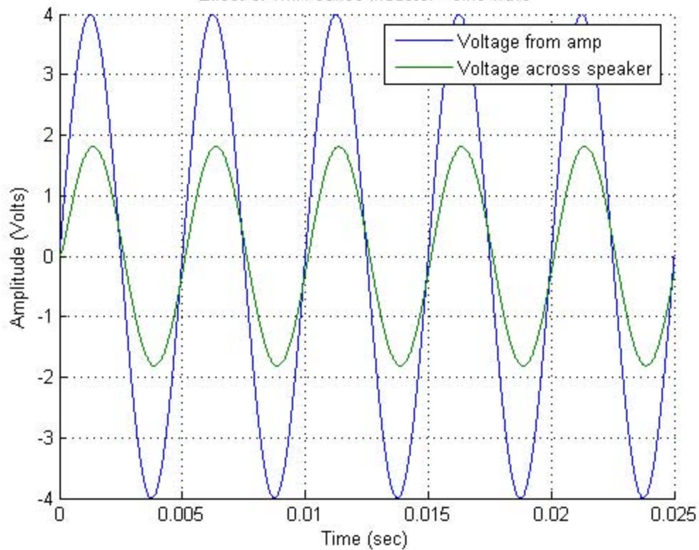
Effect of 1mH series inductor - sine wave
