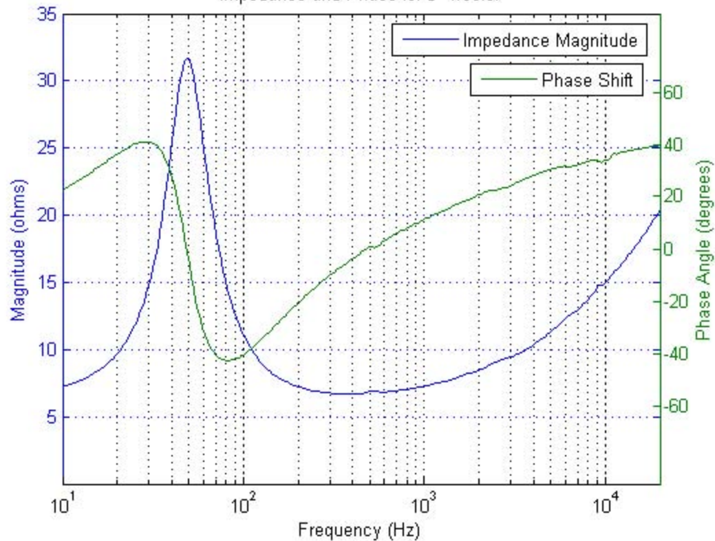
Impedance and Phase for 6" woofer
