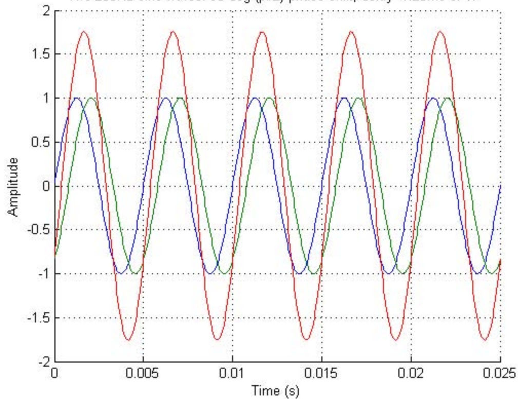
Two 200Hz sine waves: 90 deg ( \pi/2 ) phase shift; delay=1.25ms or 17°
