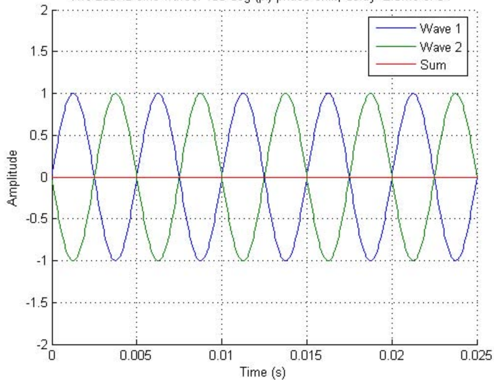
Two 200Hz sine waves: 180 deg ( \pi ) phase shift; delay=2.5ms or 34^\circ
