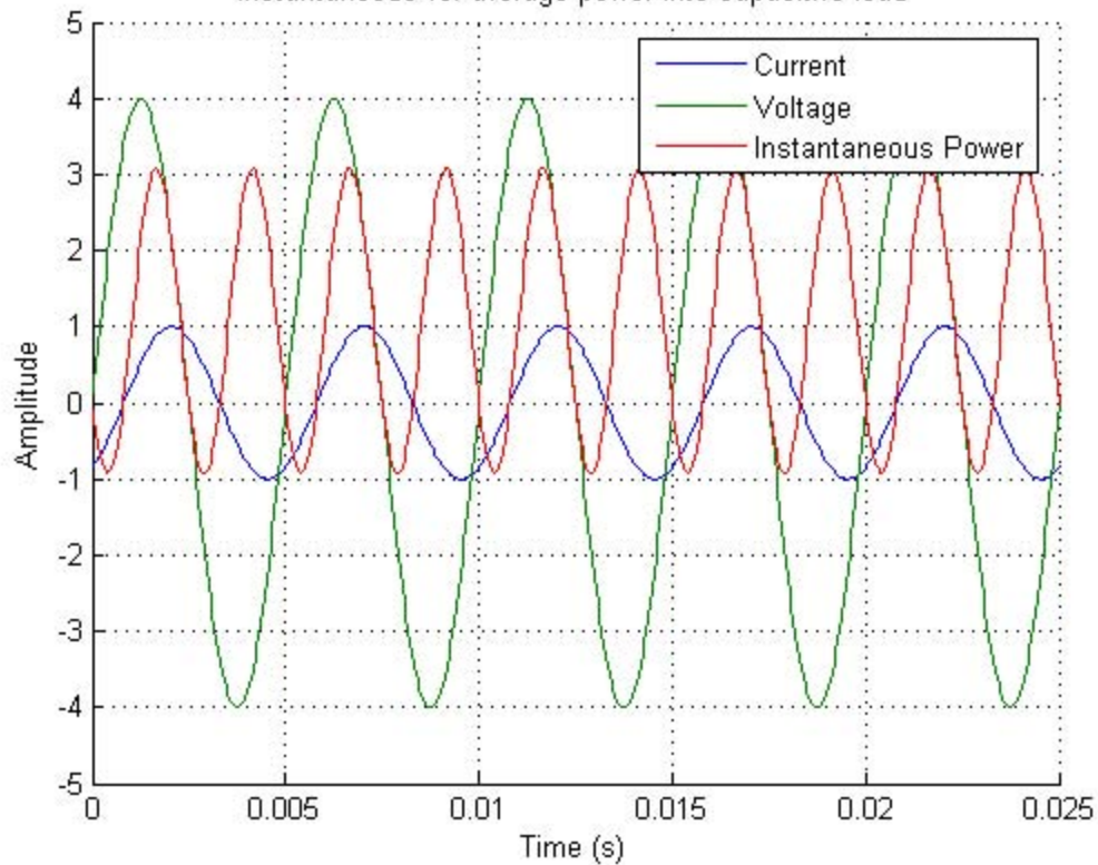
Instantaneous vs. average power into capacitive load
