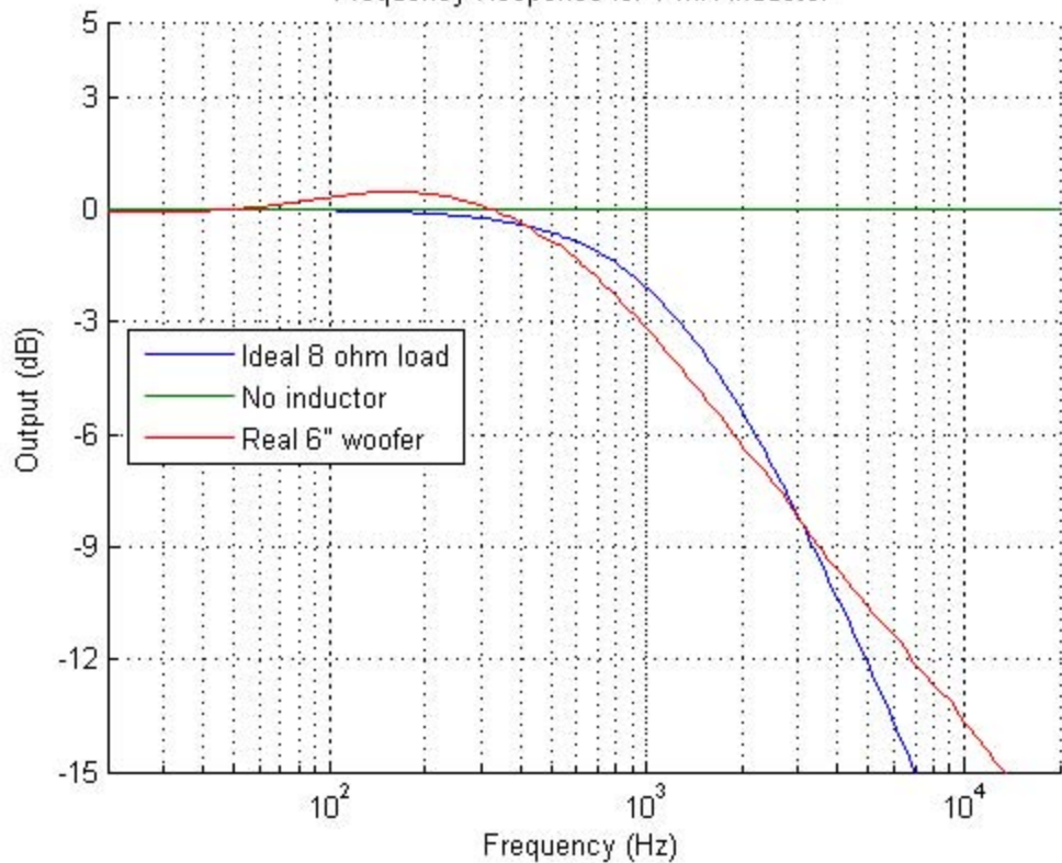
Frequency Response for 1 mH inductor
