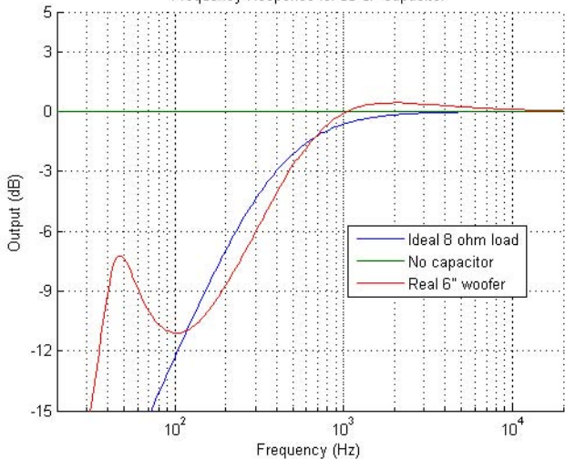
Frequency Response for 50 uF capacitor
