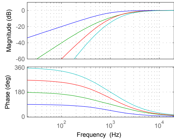
Butterworth HP ( Q = 0.707 ) filters at 1 kHz: 1st through 4th order
