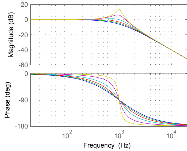
2nd order LP filters at 1 kHz: varying Q
