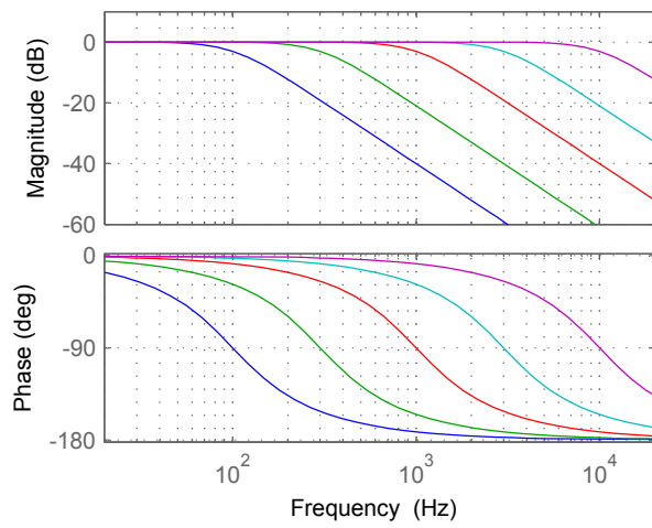
2nd order LP ( Q = 0.707 ) filters: varying corner frequency
