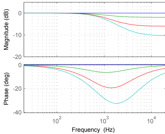
High-cut shelf filters at 1 kHz: varying shelf size
