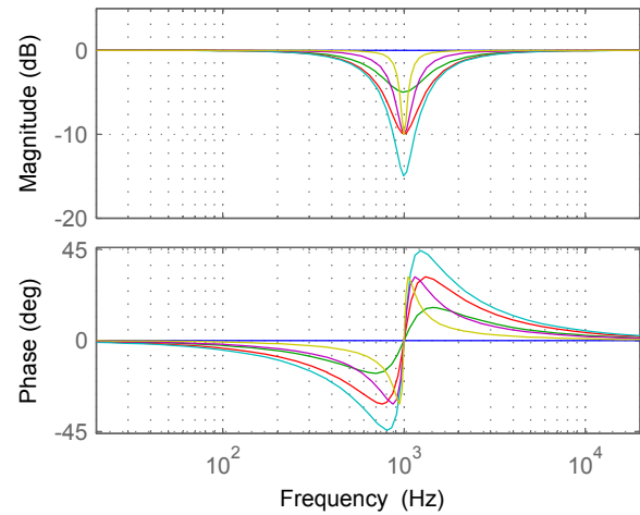
Notch filters at 1 kHz: varying Q and depth
