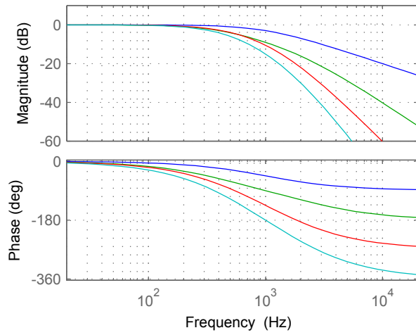
Butterworth LP ( Q = 0.707 ) filters at 1 kHz: 1st through 4th order
