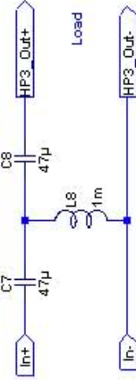
Third-order highpass (HP3)
