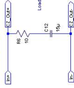
Conjugate zobel (flattens out inductive rise)
