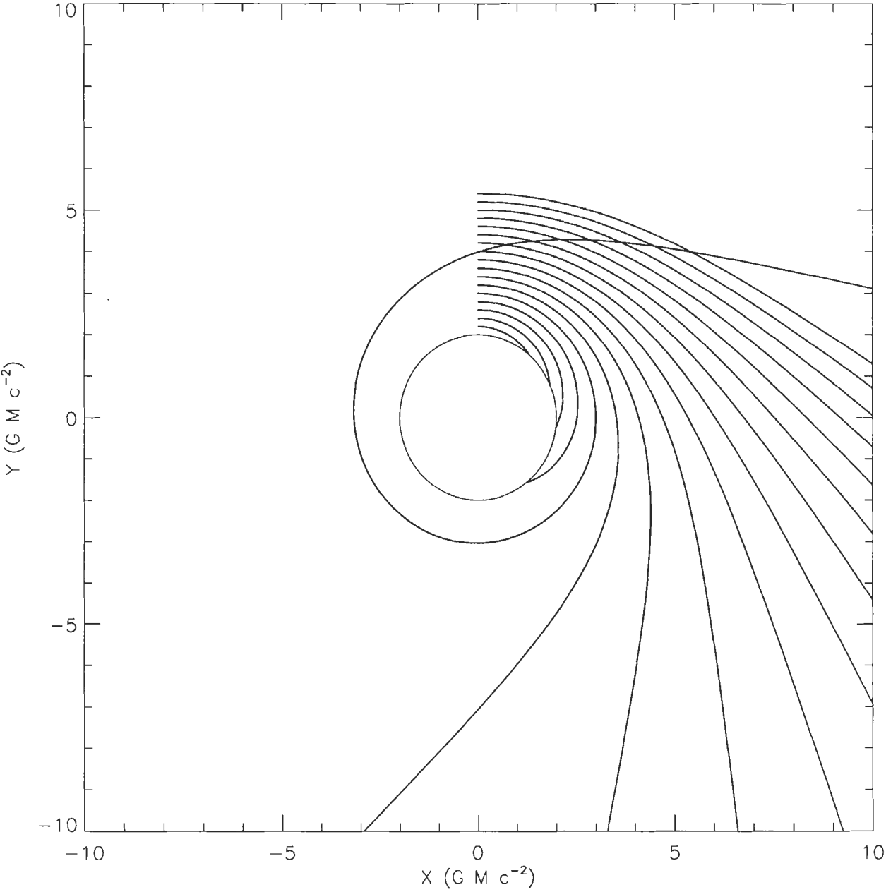
Photons leaving at right angles to the Y-axis
