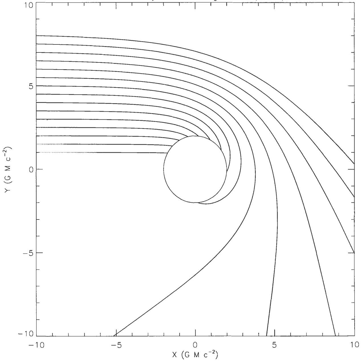
Photons from infinity with a range of impact parameters
