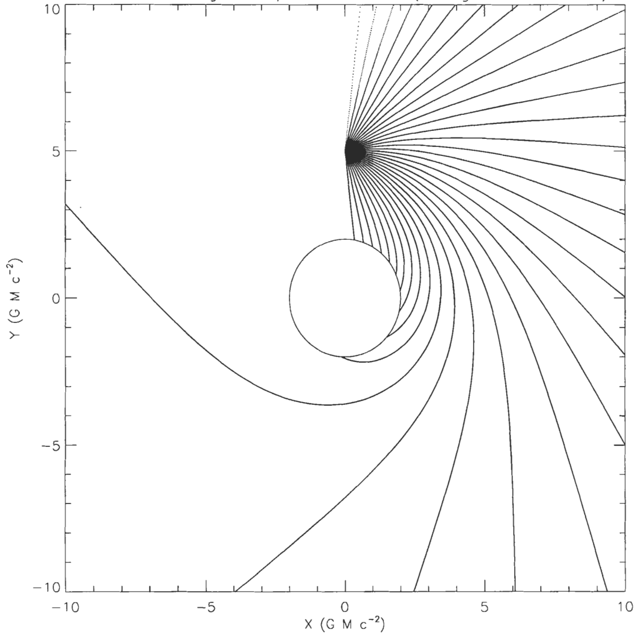
Photons leaving from point at Y=5.0 (5 degree increments)
