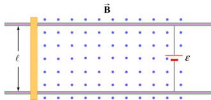
Figure 10.11.1 Sliding bar
