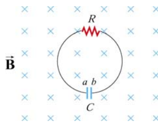
Figure 10.11.3 RC circuit in a magnetic field
