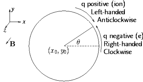
Figure 2.2: Gyro center (x_0, y_0) and orbit
