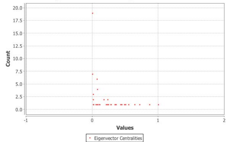
Eigenvector Centrality Distribution
