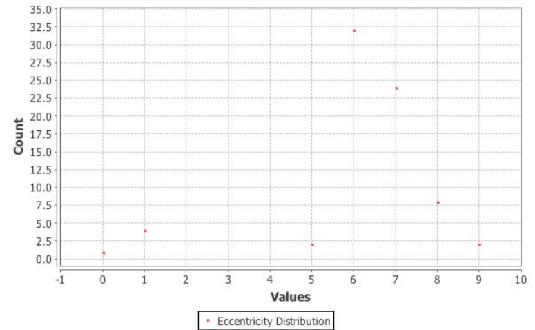
Eccentricity Distribution
