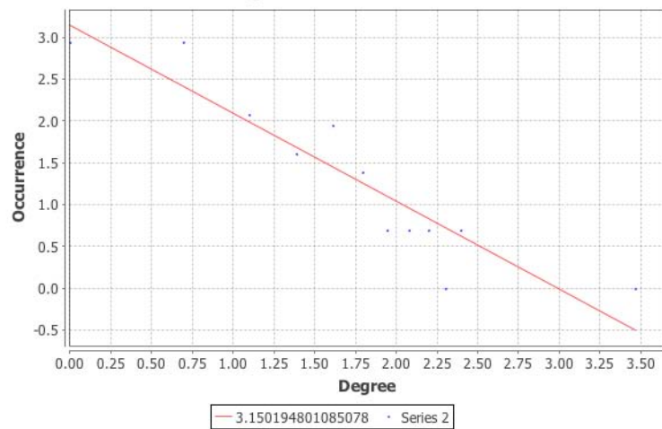
Degree Distribution
