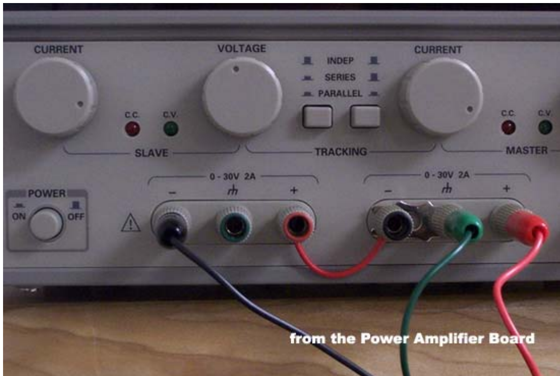
LVDT Conditioner hookup:
