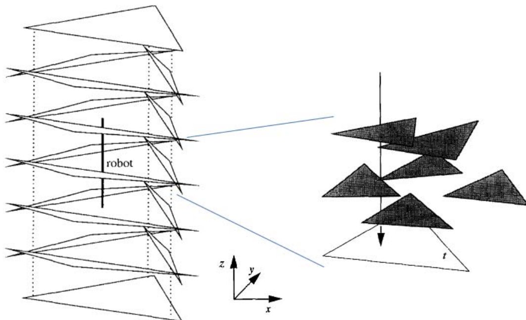
Figure 10: 3D motion planning.
