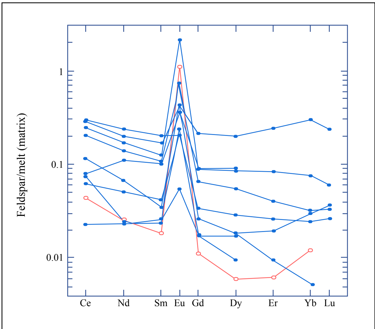
Figure 16. REE partition coefficients for (plagioclase phenocryst)/matrix (solid circles) and (K-feldspar phenocryst)/matrix (open circles). Note the overall negative slope, the range in absolute values and the peak at Eu, known as the Eu anomaly. This anomaly is a result of preferential incorporation of Eu +2 into feldspar. Figure from Schnetzler and Philpotts, 1970.
