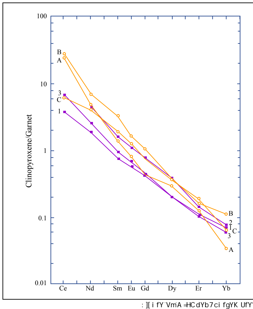
Figure 18. REE partitioning between coexisting clinopyroxene and garnet in garnet lherzolites (from Shimizu, 1975).
