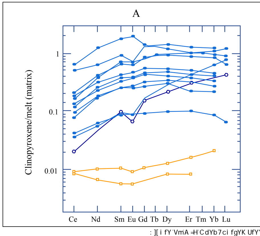
Figure 14. (Clinopyroxene phenocryst)/matrix estimates of REE partition coefficients; filled circles indicate CaO-rich clinopyroxene and open circle indicates data for a CaO-poor pyroxene, known as pigeonite. Also shown are data for (olivine/phenocryst)/matrix estimates of REE partition coefficients (open squares). Figure adapted from Schnetzler and Philpotts (1970).
