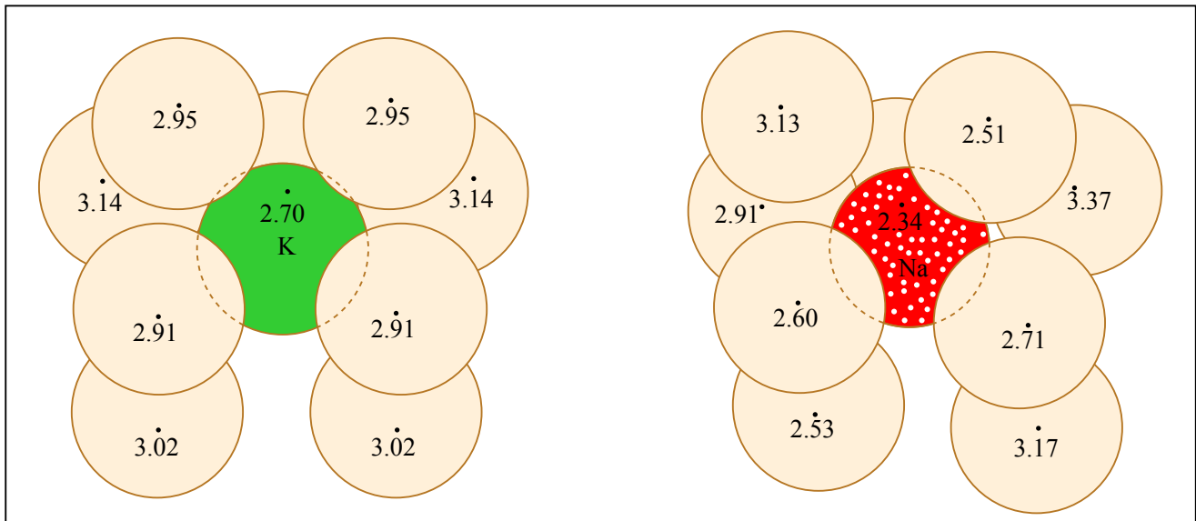
Figure 15. Oxygen coordination (CN=9) around K +1 in sanidine (left) and Na +1 in albite (right). Numbers indicate K-O and Na-O distances in angstroms (10 -8 cm). Figure adapted from Figure 10 of Ribbe, 1983.
