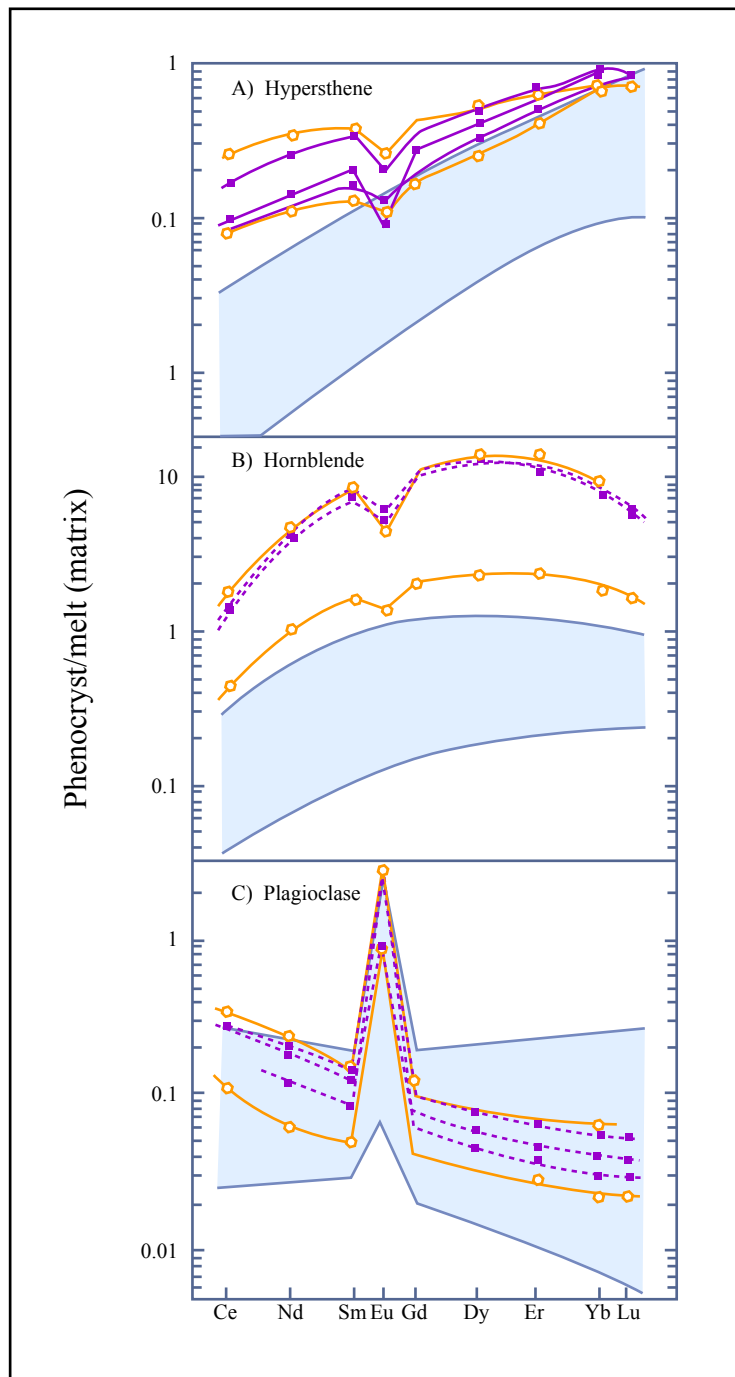
Figure 19. Data points indicate phenocryst/dacitic matrix partition coefficients; shaded fields indicate range for basaltic and andesitic matrices. No difference is observed for plagioclase but hypersthene (orthopyroxene) and amphibole partition coefficients are notably larger for the dacitic matrix. As an aside, REE partition coefficients for amphibole (hornblende) are similar to those for clinopyroxene in both a relative and absolute sense (compare with Figure 14c). The figure is from Nagasawa and Schntzler (1971).
