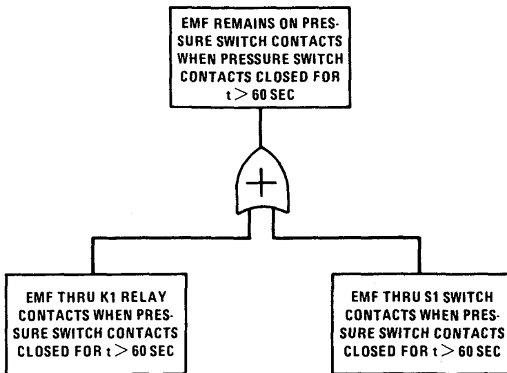
Figure VIII-10. Fault Tree Construction – Step 8
