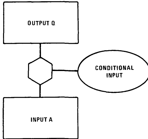
Figure IV-8. The INHIBIT-Gate
