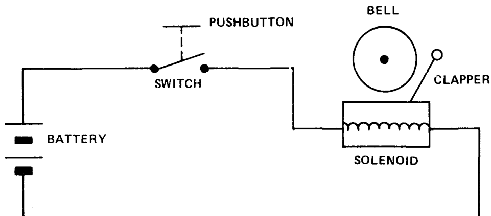
Figure V-1. Doorbell and Associated Circuitry
