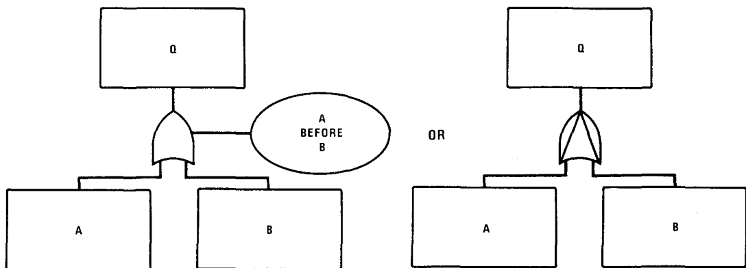
Figure IV-11. The EXCLUSIVE OR-Gate
